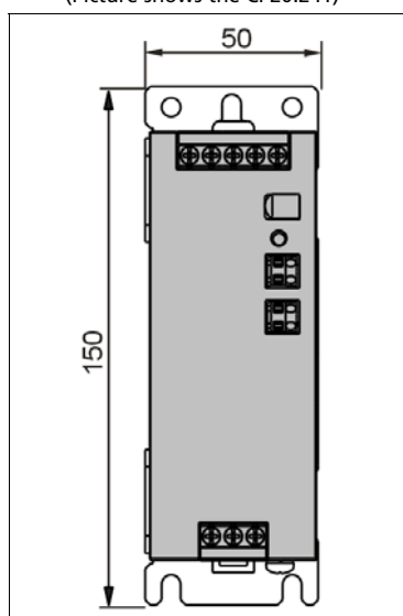
Fig. 5-3 Wall/panel mounting, front view (Picture shows the CP20.241)
