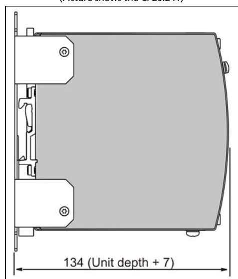
Fig. 5-5 Wall/panel mounting, side view (Picture shows the CP20.241)
