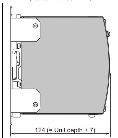
Fig. 5-5 Wall/panel mounting, side view (Picture shows the CP10.241)
