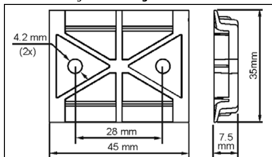
Fig. 2 Mounting dimensions
