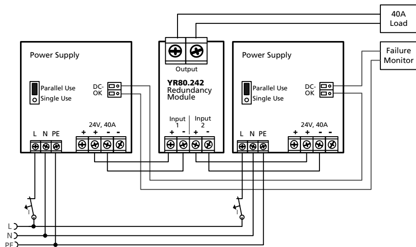
Fig. 17-1 Wiring diagram, 1+1 Redundancy, 40A output current
