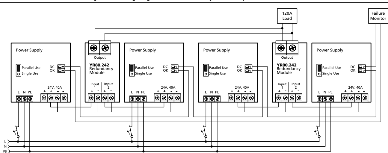
Fig. 17-2 Wiring diagram, n+1 Redundancy, 120A output current
