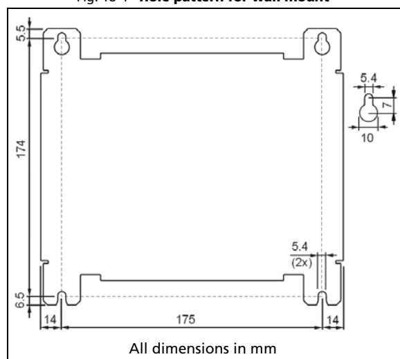
Fig. 18-4 Hole pattern for wall mount
