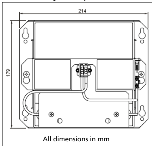
Fig. 16-1 Top view
