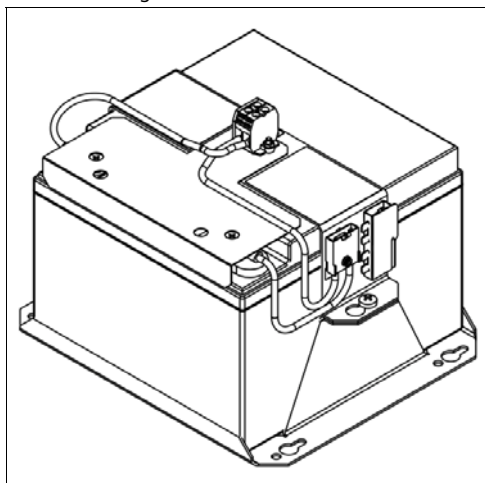
Fig. 16-3 Isometric view
