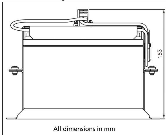
Fig. 16-2 Side view
