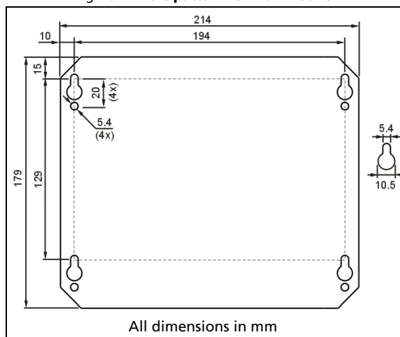
Fig. 16-4 Hole pattern for wall mount
