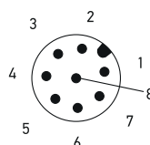
MALE M12 8 pins Safety SLS master 1708
