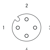
FEMALE M12 4 pins Ethernet, F, Key D
