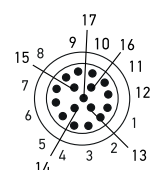
MALE M12 17 pins Safety SLS master 1708
