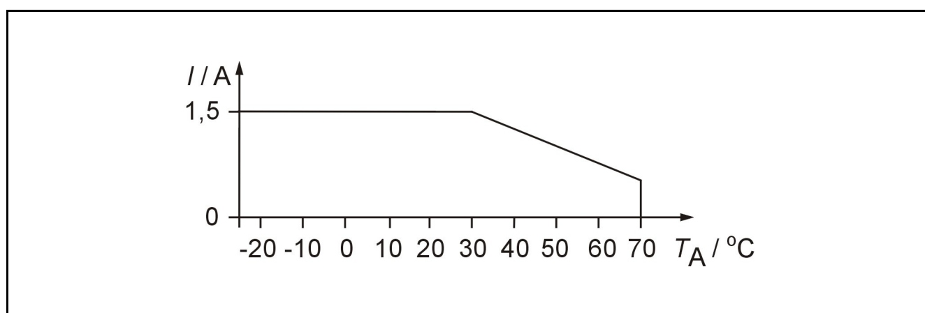
Derating curve for SLO P230TR.
