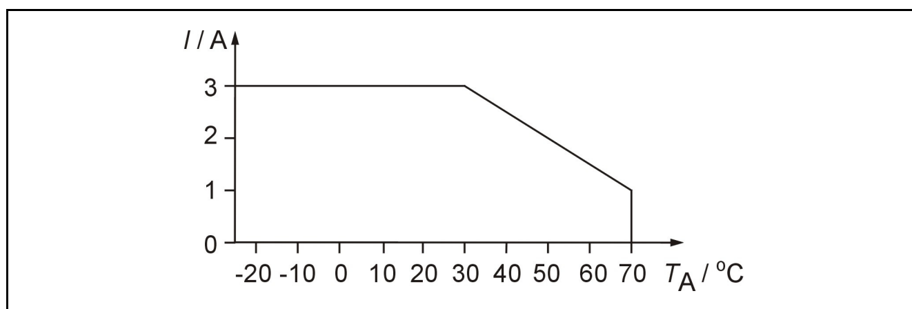
Derating curve for SLO P120TR.
