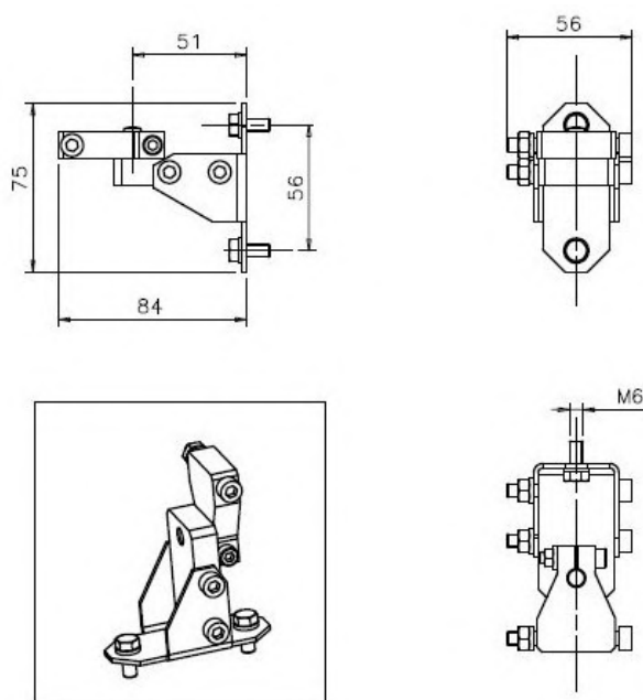
Figure 23 - Mounting kit
