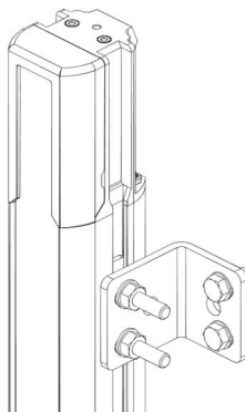
Figure 20: Fixing with two screws
