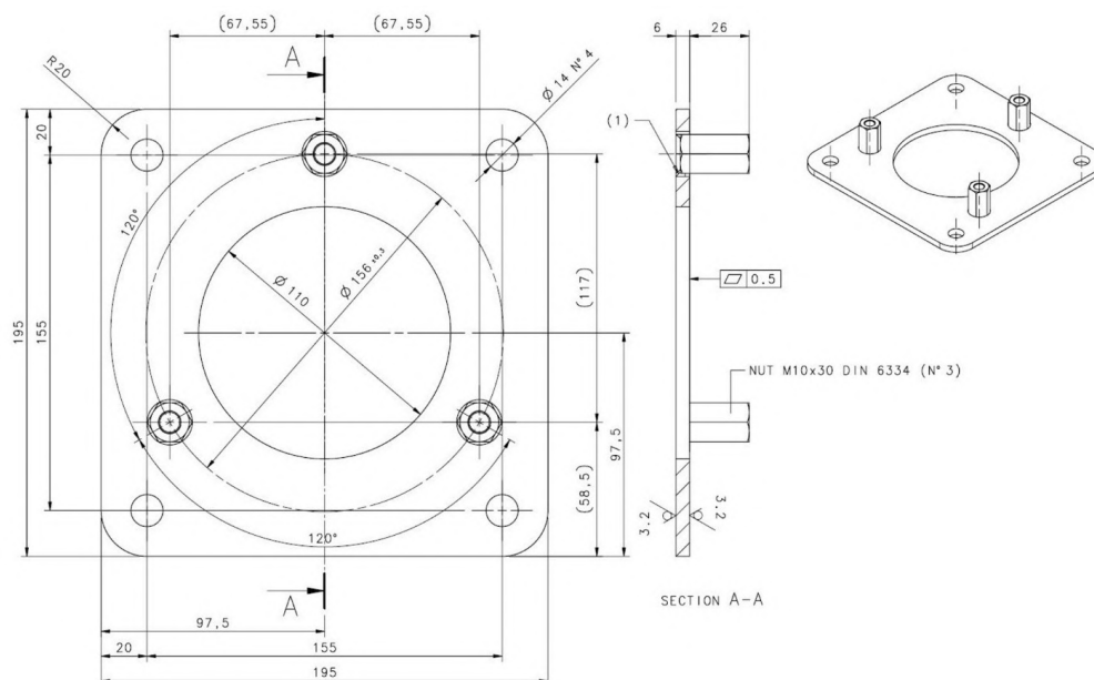
Figure 18 - Plate kit
