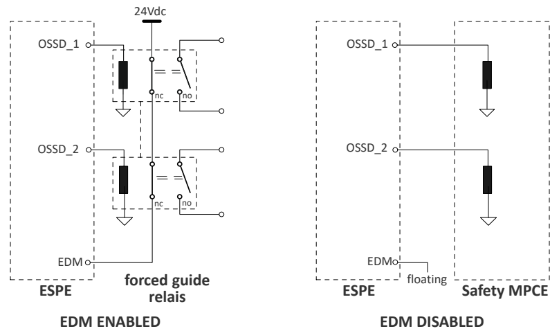
Figure 9: EDM wiring
