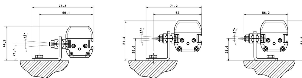
Figure 10 - Angled fixing bracket + Orientable support
