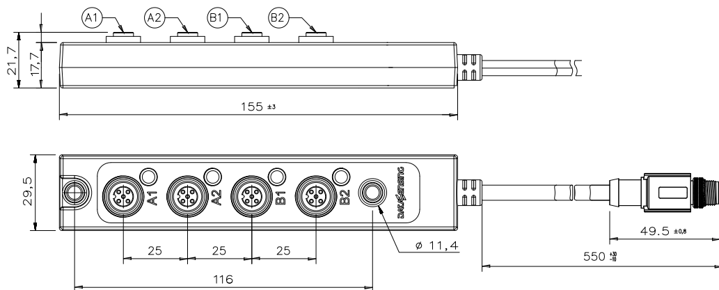
Figure 29 - Dimensions (mm)
