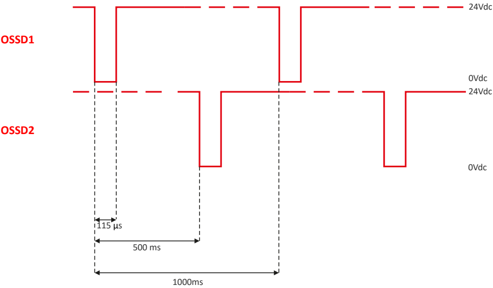
Figure 4: Behavior of OSSDs
