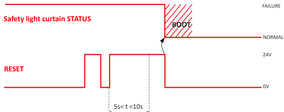
Figure 8: Reset function timing
