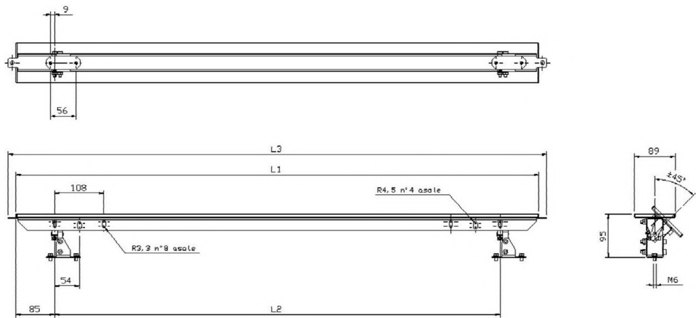
Figure 21 - Deviating mirrors (mm)
