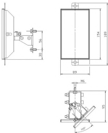
Figure 22 - SG-DM 150 (mm)
