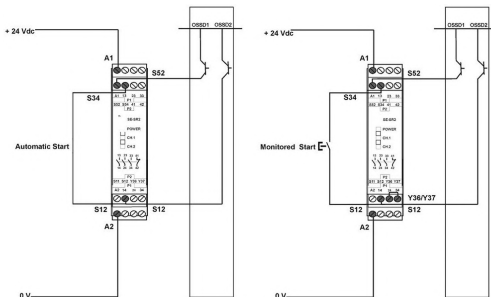
Figure 26 - Safety relay
