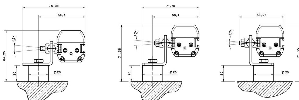
Figure 12 - Angled fixing bracket + Orientable support + Anti-vibration support
