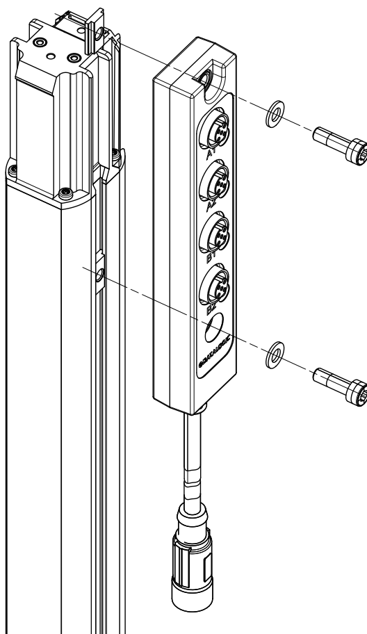
Figure 28 - Connection box
