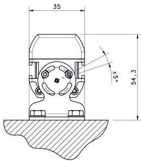
Figure 14 - Straight mounting
