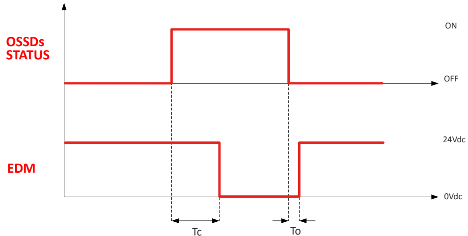
Figure 10: EDM function timing
