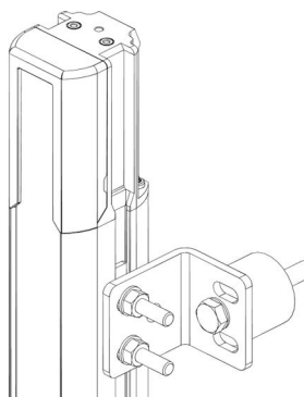
Figure 22: Anti-vibration dampers
