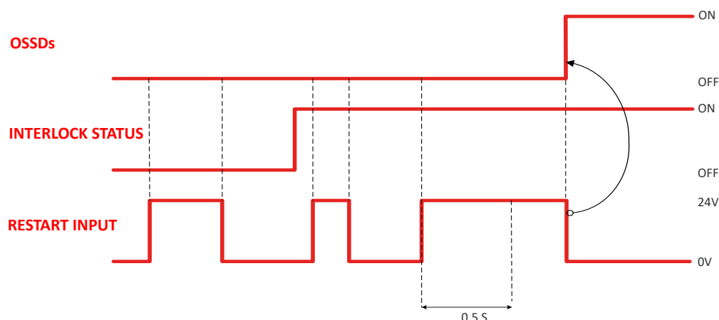
Figure 7: OSSDs behavior in Manual Restart Mode and Restart Pattern
