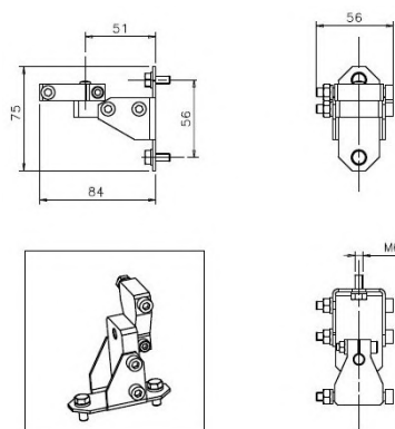
Figure 24 - Mounting kit
