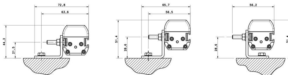
Figure 9 - Angled fixing bracket
