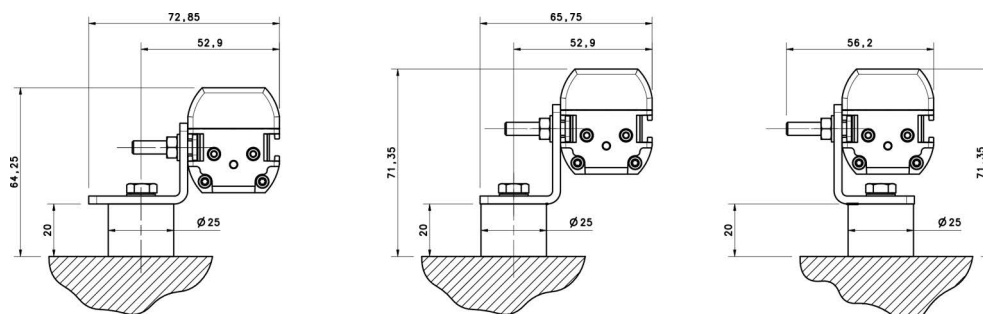
Figure 11 - Angled fixing bracket + Anti-vibration support
