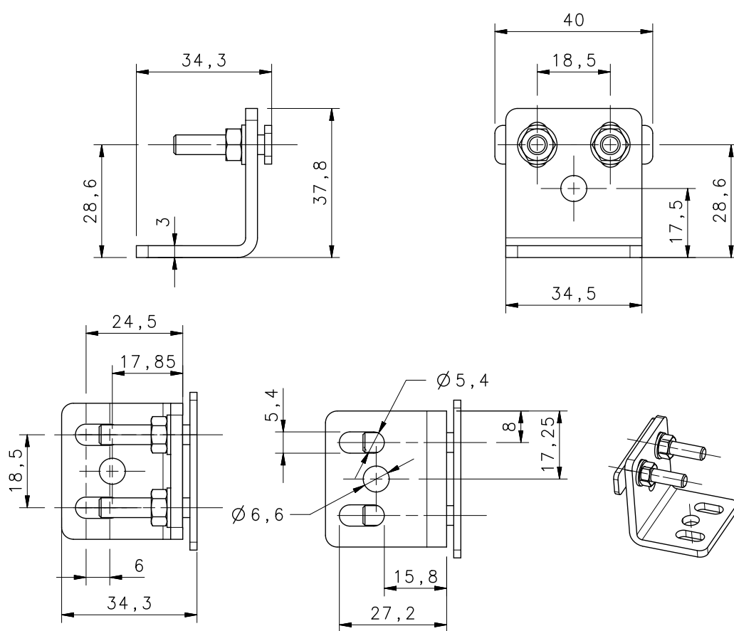
Figure 7 - Metal Angled fixing Bracket
