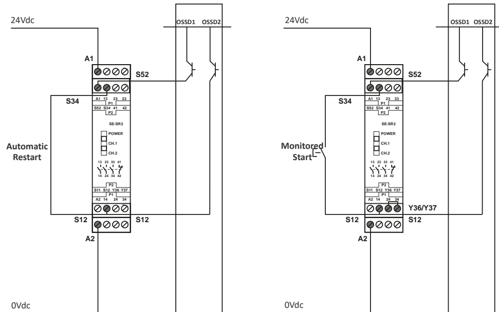
Figure 2: Connection to SE-SR2 Safety Relays
