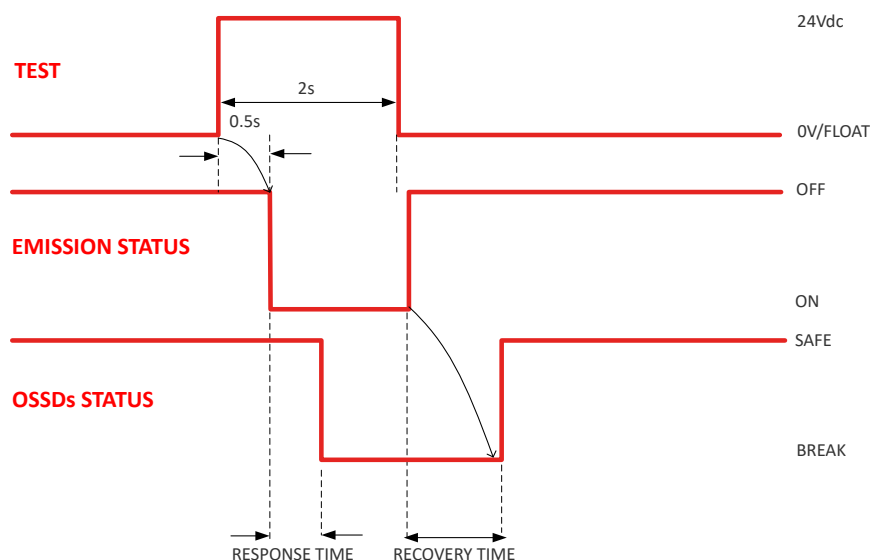
Figure 11: OSSDs timing for test on TX
