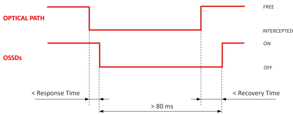
Figure 6: OSSDs behavior in Automatic Restart mode
