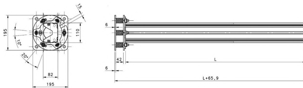
Figure 19 - Mounting with SG-P SB
