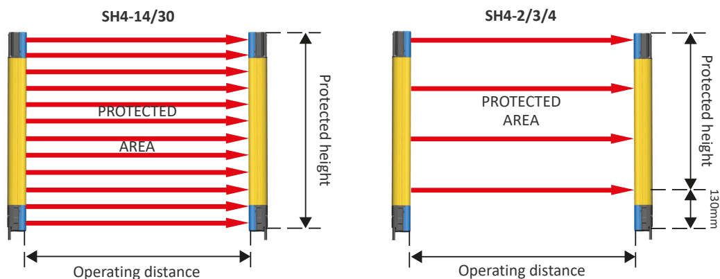
Figure 2: Detection zone
