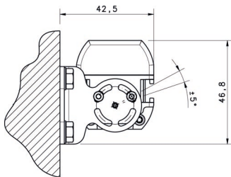
Figure 15 - Rotating 90° mounting
