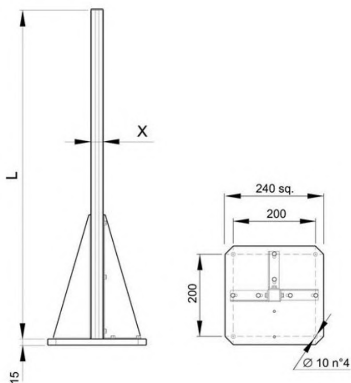
Figure 20 - Dimensions (mm)
