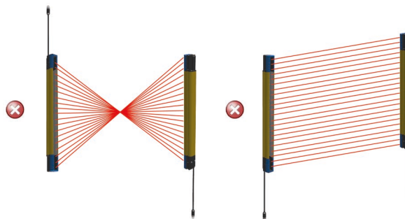
Figure 14: Wrong light curtain TX-RX orientations
