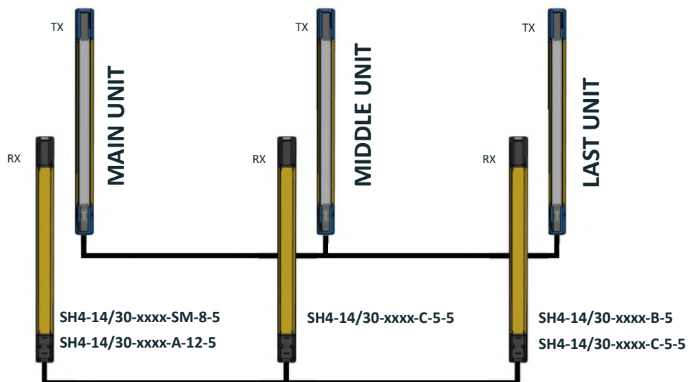
Figure 31: Cascade system
