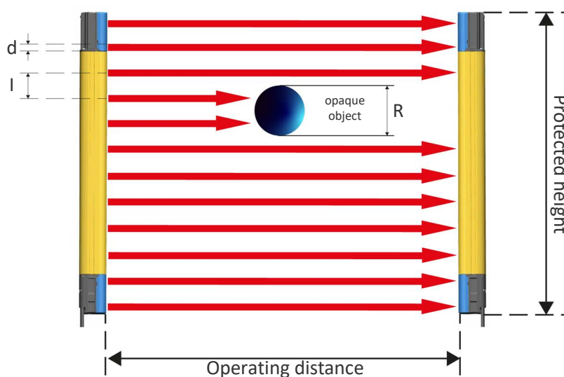
Figure 1: Detection capability
