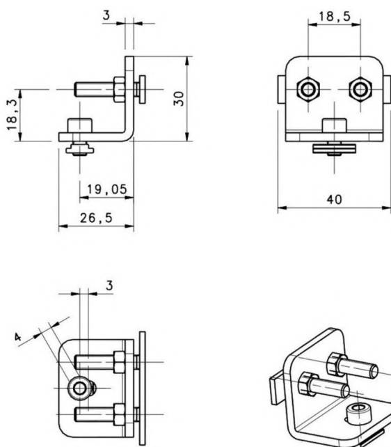
Figure 17 - Mounting kit
