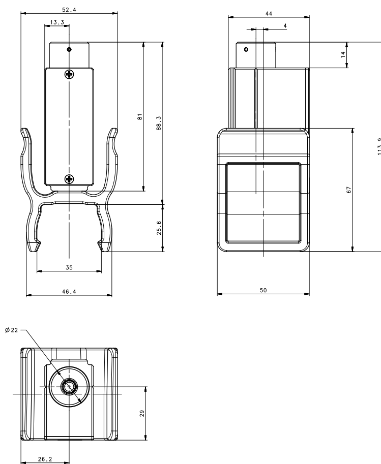
Figure 25 - Dimensions (mm)
