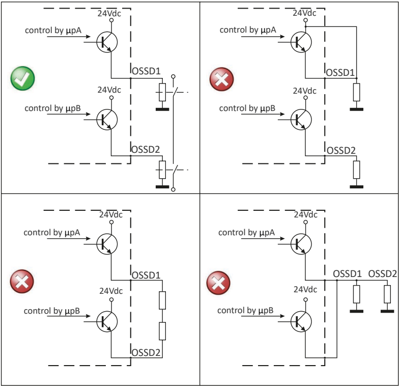
Figure 3: OSSDs connection
