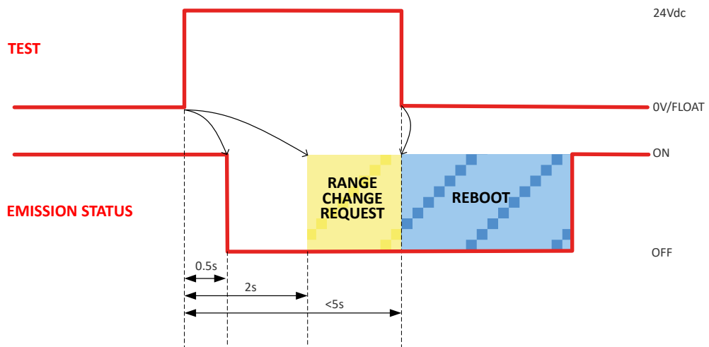
Figure 12: Emission Range Change Request timings
