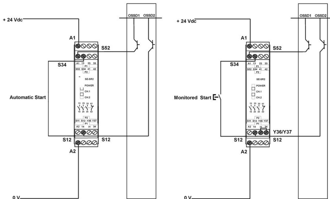
Fig 29 - Safety relay
