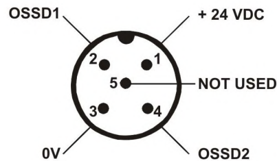
Fig 19 - Receiver
