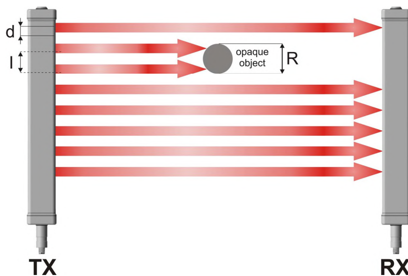
Fig 1 - Detection capability
