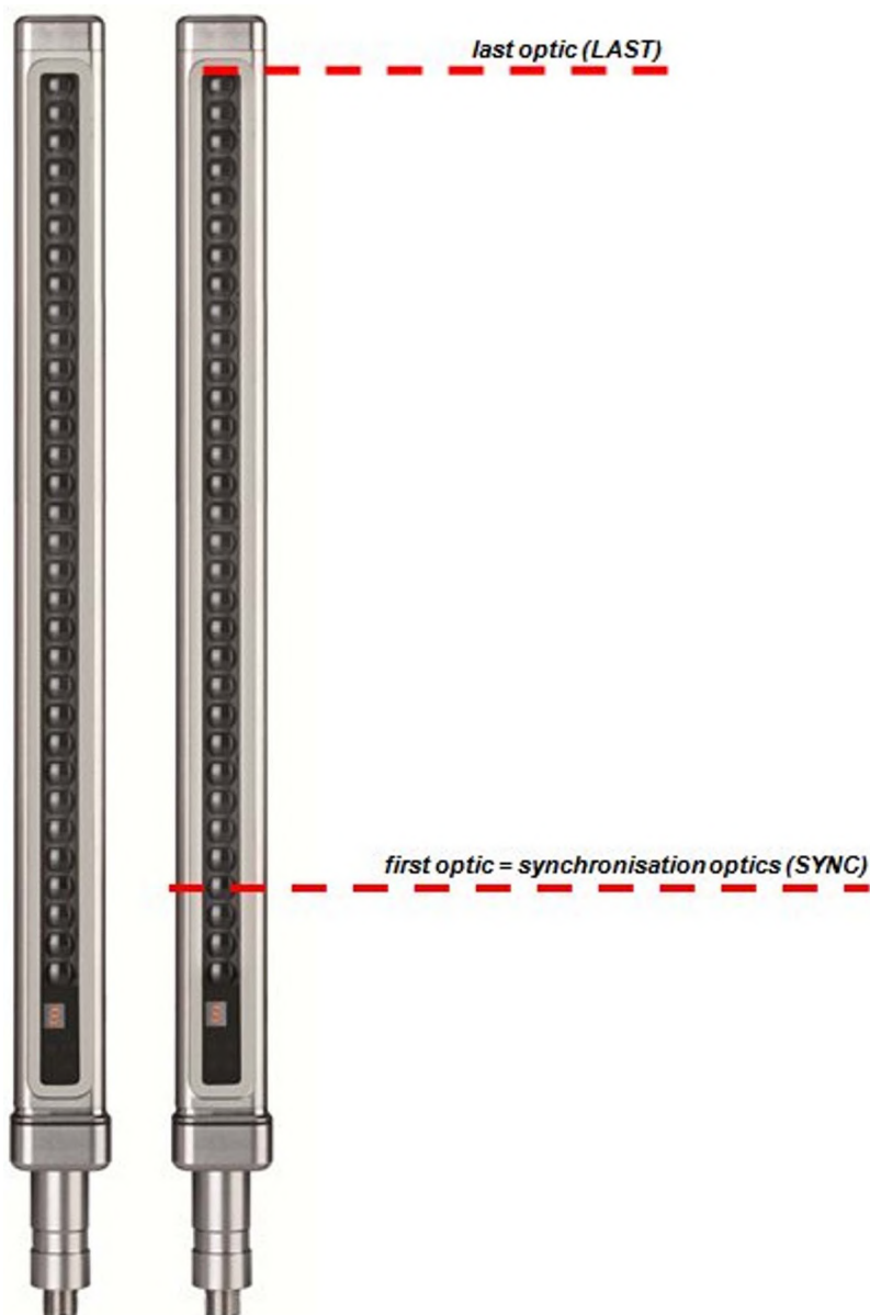
Fig 24 - SYNC optics
