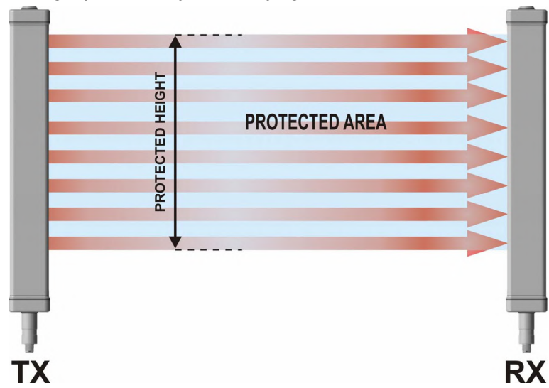
Fig 2 - Detection Zone
