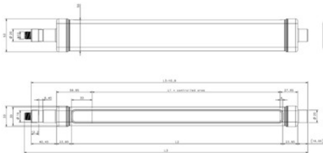
Fig 28 - Overall dimensions (mm)
