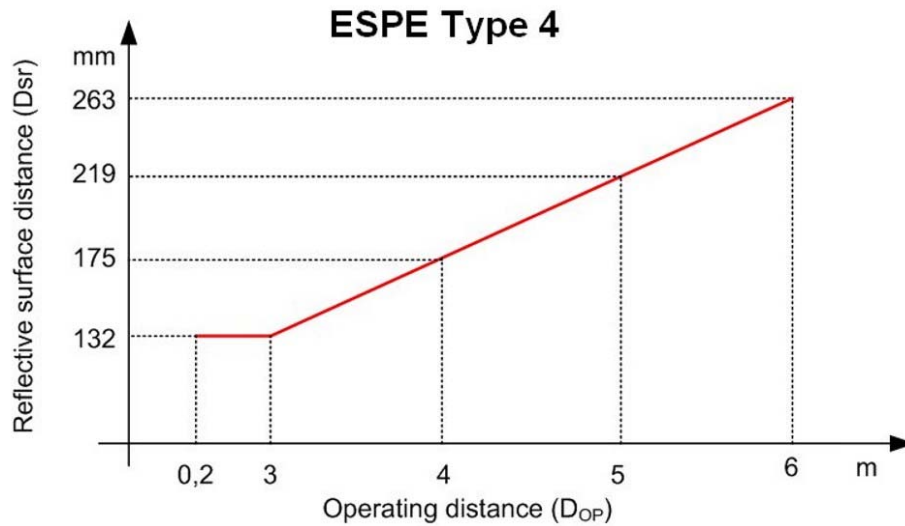
Fig 12 - Minimum distance from reflective surface
