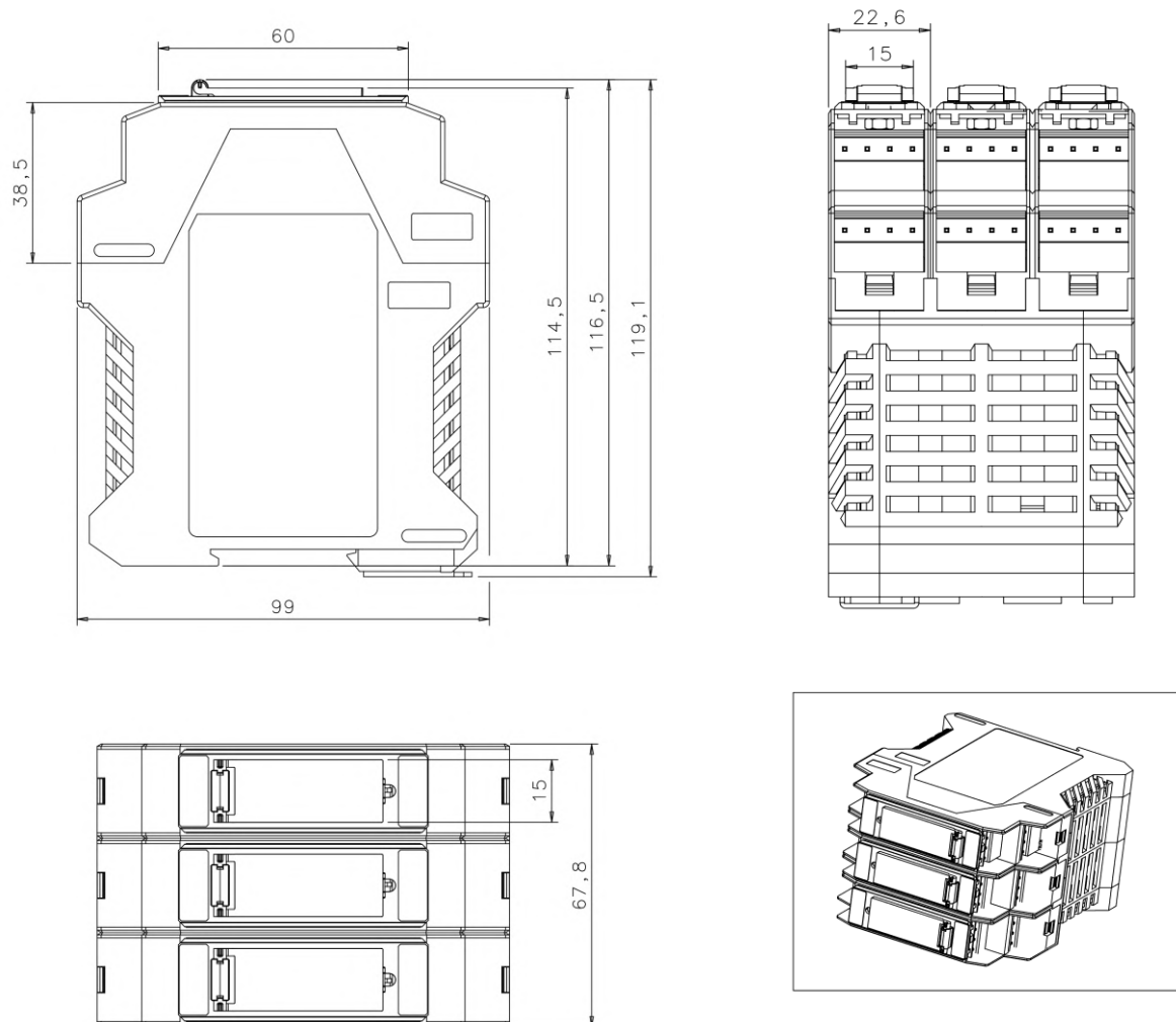
Fig. 38 SG-BWS-T4-MT overall dimensions
