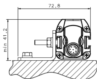
MOUNTING A
