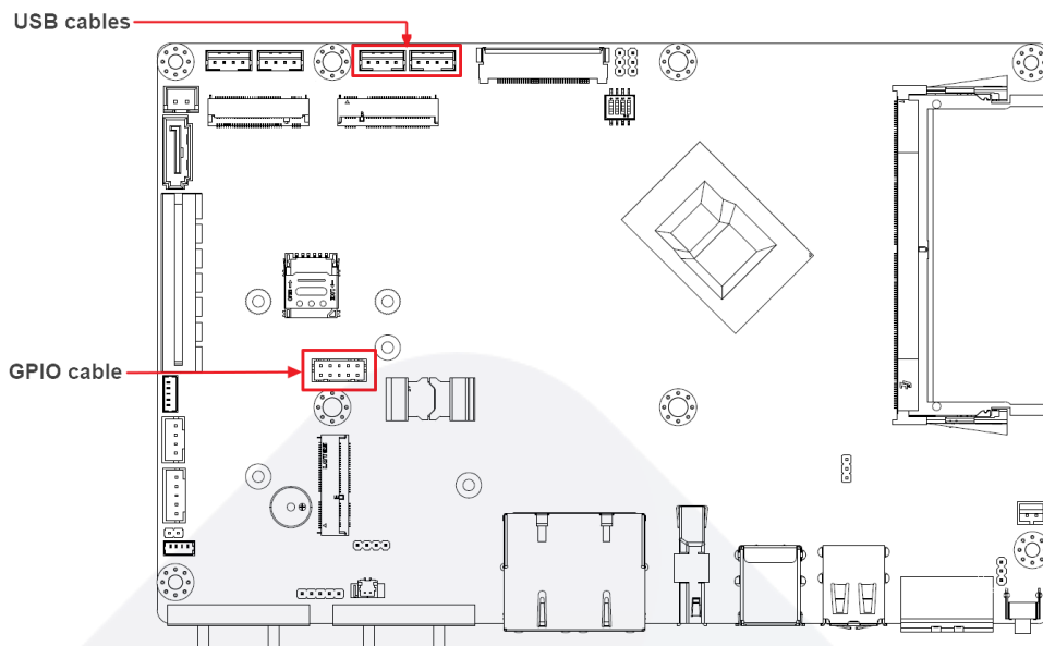
Figure 2.8 GPIO and USB Connectors
