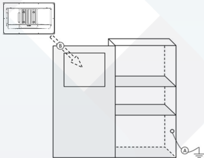
Figure 2.20 Cabinet Installation
