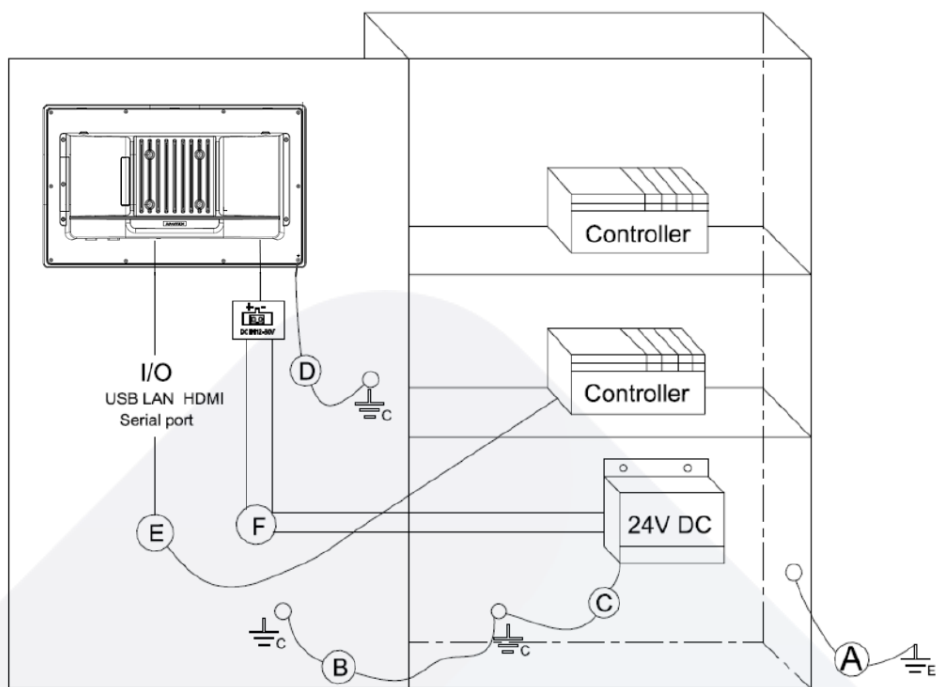
Figure 2.21 System Wiring
