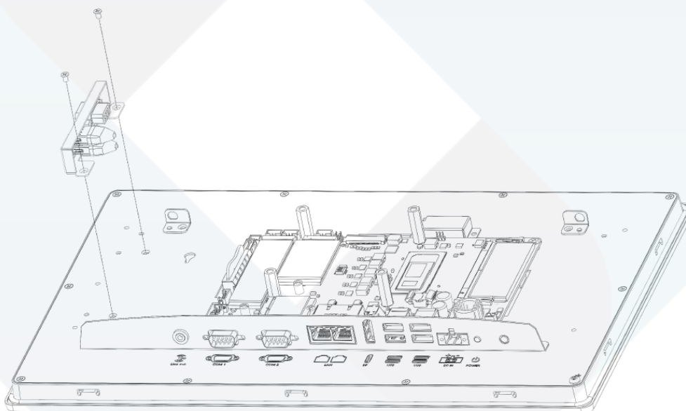
Figure 2.7 GPIO+USB Module Installation
