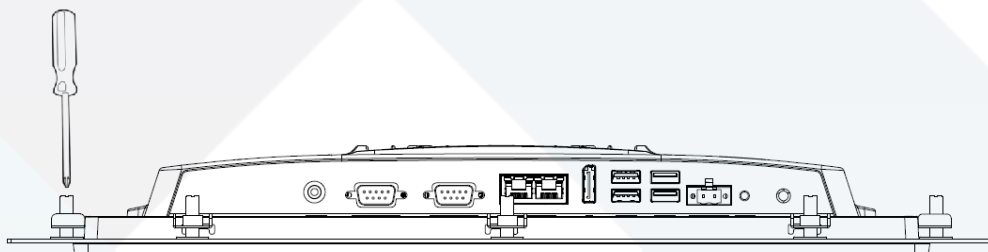
Figure 2.18 Panel Mounting (2)
