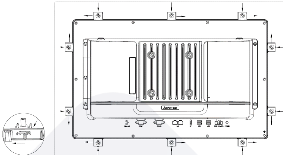
Figure 2.17 Panel Mounting (1)
