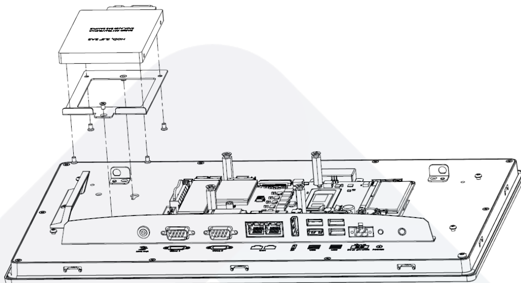
Figure 2.4 SSD Installation
