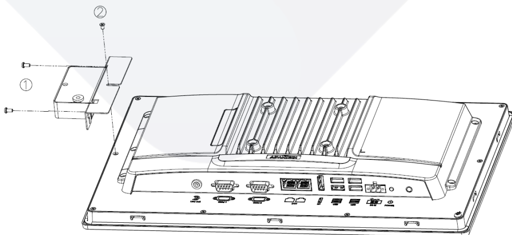
Figure 2.15 RFID Reader Installation
