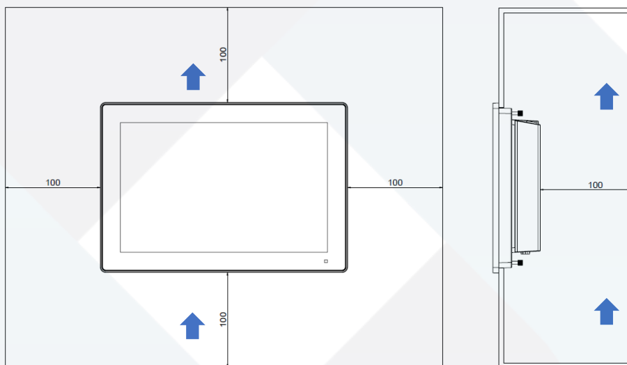
Figure 2.16 Panel Mounting – Positioning
