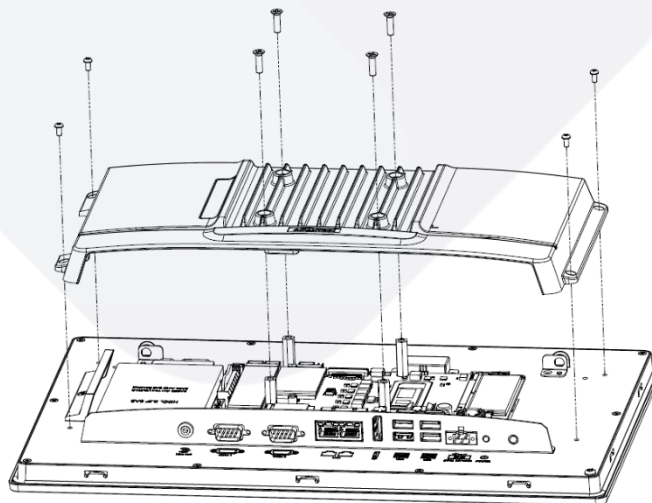
Figure 2.3 Rear Cover Removal
