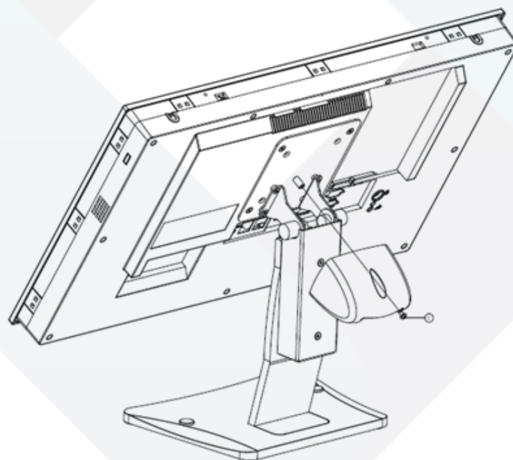
Figure 2.21 Securing the Stand Mount Hinge Cover
