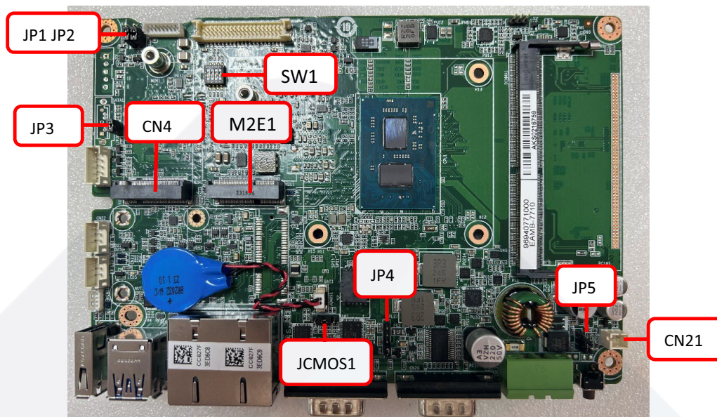
Figure 3.1 Motherboard
