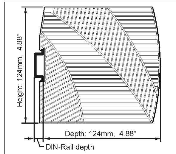
Fig. 20-2 Side view
