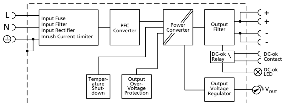
Fig. 11-1 Functional diagram PIC240.241D
