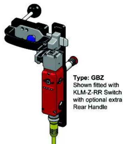
Type: GBZ Shown fitted with KLM-Z-RR Switch with optional extra Rear Handle
