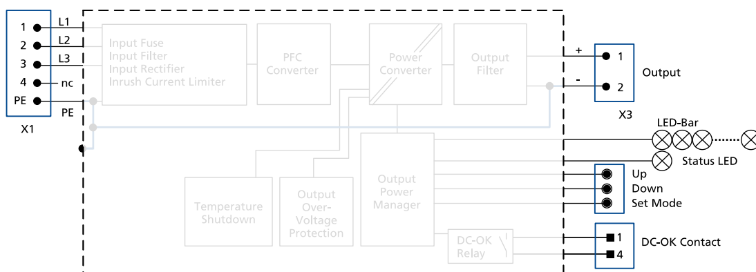
Fig. 12-3: Functional Diagram FPT500.241-010-108
