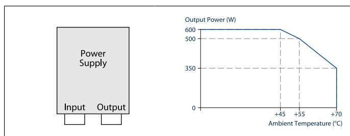
A Standard Orientation
