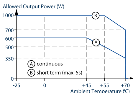
Fig. 16-1: Output power vs. ambient temp.
