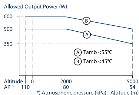
Fig. 16-2: Output power vs. ambient temp.
