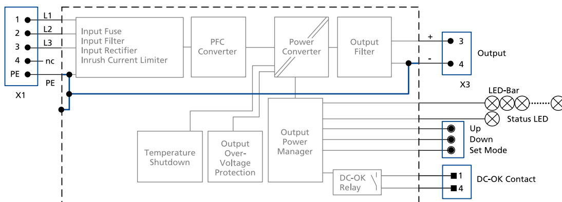
Fig. 12-1: Functional Diagram FPT500.241-002-101
