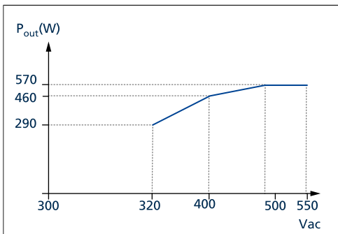
Fig. 23-1: Two phase power capability
