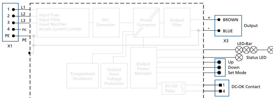
Fig. 12-2: Functional Diagram FPT500.241-006-104
