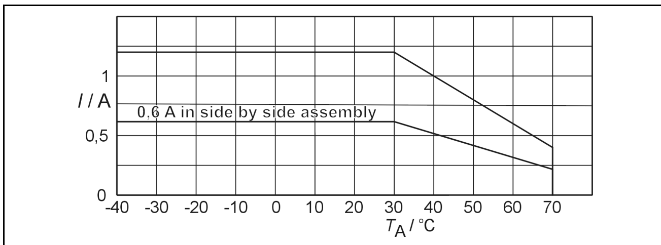
Derating curve for SLO 24IRA.
