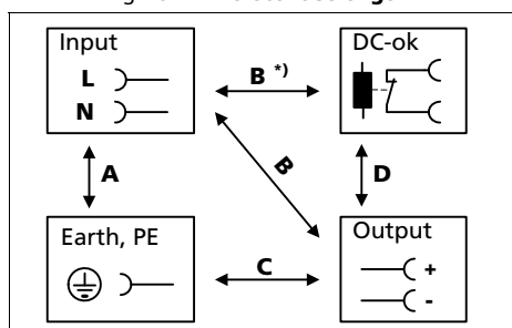
Fig. 19-1 Dielectric strength
