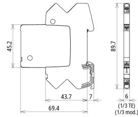
Dimension drawing BCO ML2 BD EX 24
