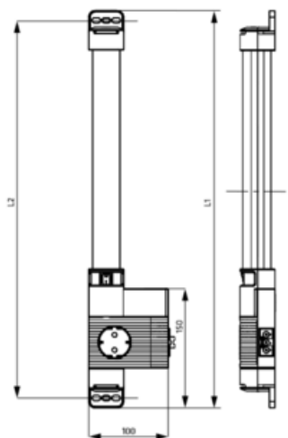
LED 121 (Size 1) L1 = 500 mm L2 = 475 mm LED 122 (Size 2) L1 = 700 mm L2 = 675 mm
