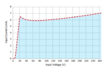
Input current vs Input Voltage Standard Regulated AC/DC inputs
