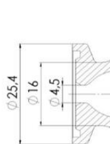
Micro flange
