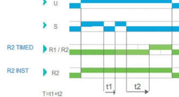
Function At - Summation time relay
