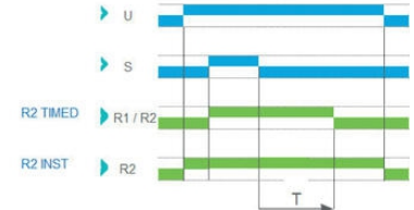
Function C - Off-Delay (Delay on break)
