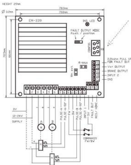
EM-339 WIRING EXAMPLES
