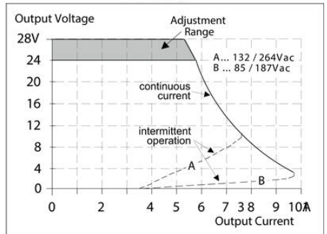
Fig. 6-1 Output voltage vs. output current, RMS current, typ.
