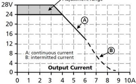
Output Voltage
