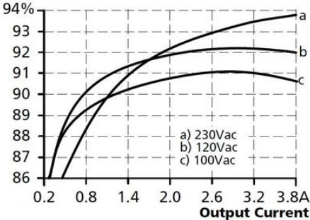
Efficiency
