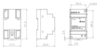
CHROME Chrome DIN Rail Power Supply 24V 30W 1 Phase / DRC-24V30W1AZ
