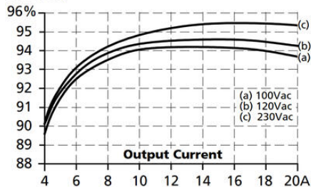
Efficiency
