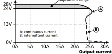
Output voltage
