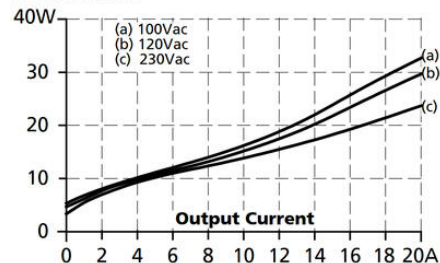
Power Losses
