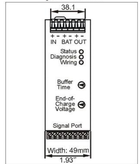
Fig. 24-2 Front view
