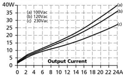
Power Losses
