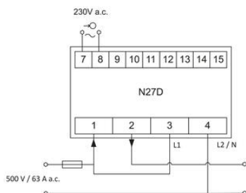
Connection diagram
