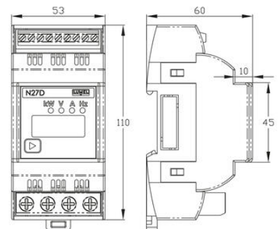
External dimensions
