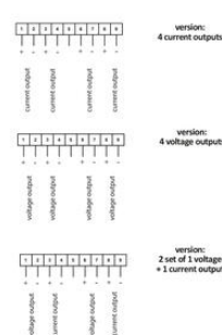
Fig. 2 Analog outputs versions.
