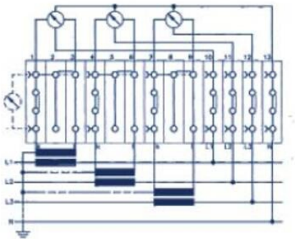
3-phase with voltage disconnects
