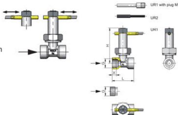
UR1 with plug M12x1
