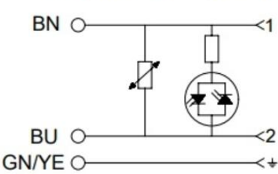
ELECTRICAL DIAGRAM C4
