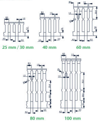
Dimensional drawings Height / side profile
