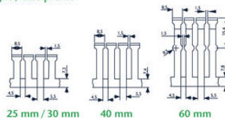
Dimensional drawings Height / side profile
