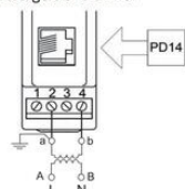
f) indirect measurement of frequency by means of voltage transformer
