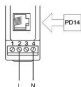
a) indirect measurement of voltage
