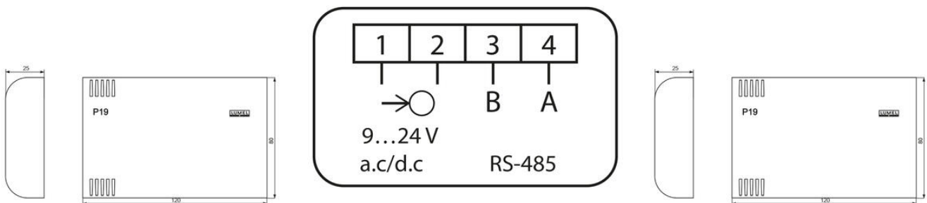
Connection diagram
