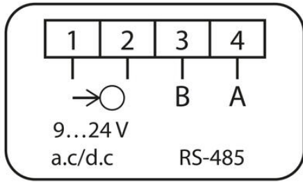
Connection diagram
