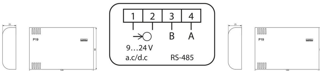
Connection diagram
