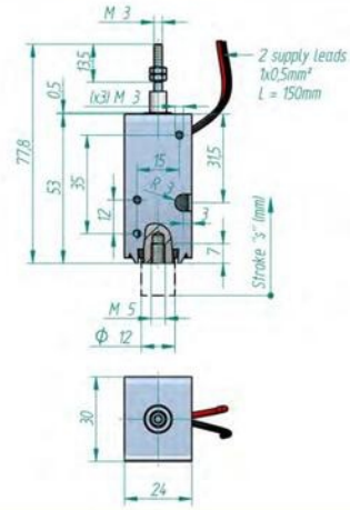
Solenoid locked
